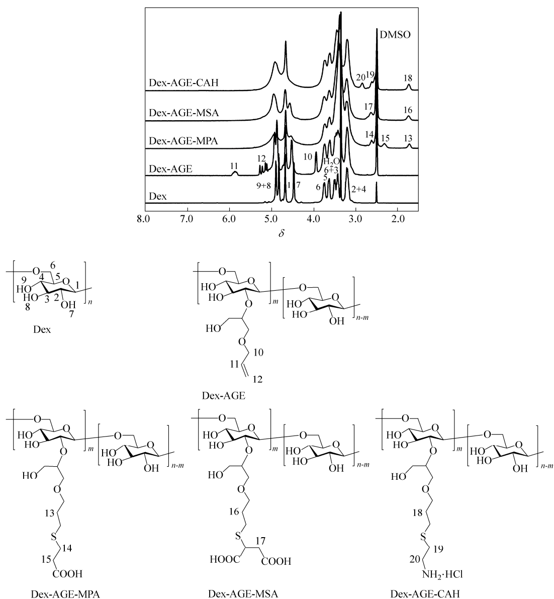
Fig. 1 Chemical structures and 1 H-NMR spectra of Dex, Dex-AGE, Dex-AGE-MPA, Dex-AGE-MSA and Dex-AGE-CAH
